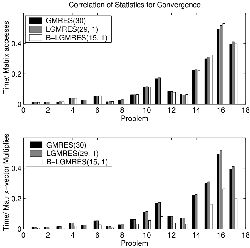
FIG. 6. The upper panel shows the ratios of execution time to number of accesses of A for GMRES (30), LGMRES(29, 1), and B-LGMRES(15, 1) on the 17 test problems in Table 1. The lower panel shows the ratios of execution time to number matrix-vector multiplies.
