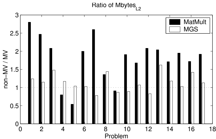
FIG. 11. A comparison of data movement from main memory to L2 cache in the MatMult and MGS sections for the non-MV implementation of B-LGMRES(15,1) versus the MV implementation for 10 restart cycles.
