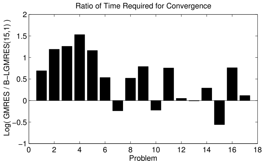
FIG. 7. A comparison of the time required for convergence with B\text{-LGMRES}(15, 1) versus full \text{GMRES} on the 17 test problems in Table 1.
