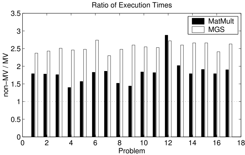
FIG. 10. A comparison of execution time for the MatMult and MGS sections with the non-MV implementation of B\text{-LGMRES}(15,1) versus the MV implementation for 10 restart cycles.
