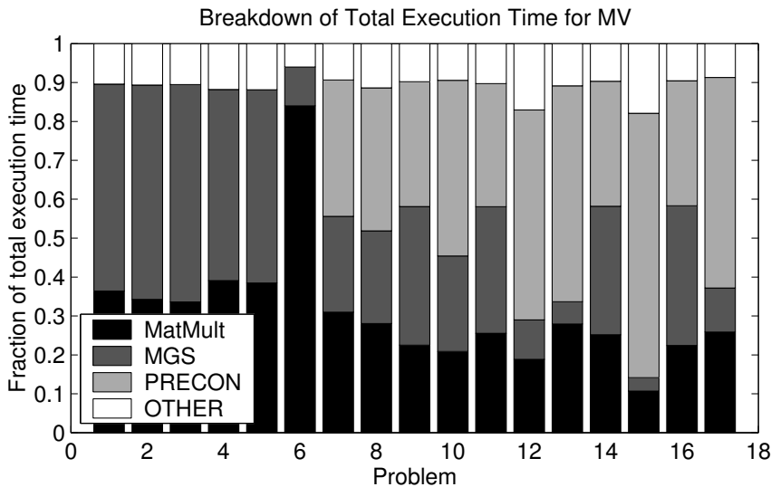
FIG. 8. Percentage of time for each section of code of the MV implementation of B-LGMRES(15,1).
