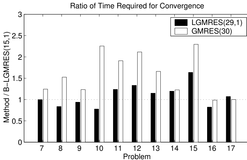
FIG. 5. A comparison of the time required for convergence for preconditioned test problems 7-17 with B-LGMRES(15, 1) versus GMRES(30) and LGMRES(29, 1). All methods use an approximation space of dimension 30, and problems are listed in order of increasing number of nonzeros.
