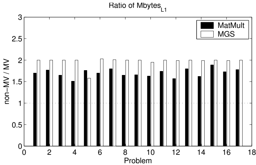
FIG. 12. A comparison of data movement from L2 cache to L1 cache in the MatMult and MGS sections for the non-MV implementation of B-LGMRES(15,1) versus the MV implementation for 10 restart cycles.
