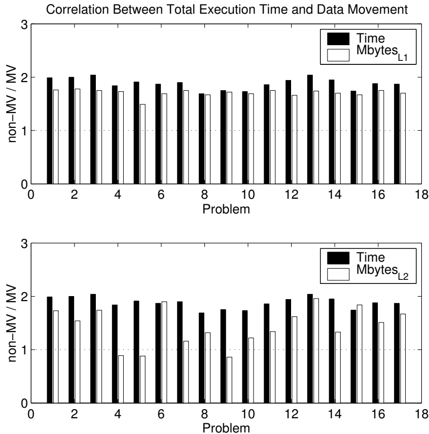
FIG. 13. The upper panel is a comparison of data movement from L2 to L1 cache in the MatMult and MGS sections for the non-MV implementation of B-LGMRES(15,1) versus the MV implementation for 10 restart cycles.. The lower panel compares data movement from main memory to L2 cache.
