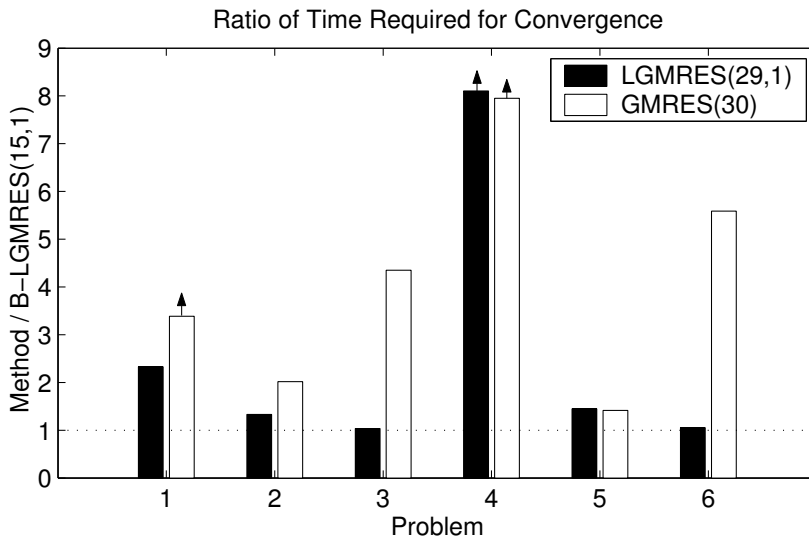
FIG. 4. A comparison of the time required for convergence for non-preconditioned test problems 1-6 with B-LGMRES(15, 1) versus GMRES(30) and LGMRES(29, 1). All methods use an approximation space of dimension 30, and problems are listed in order of increasing number of nonzeros.
